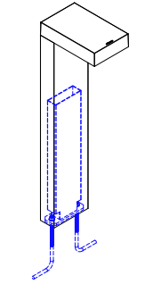
VRBI Vandal Resistant Bollard Insert This vandal resistant galvanized steel insert provides additional support and rigidity in areas with high pedestrian traffic.
