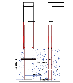
A13391 Security Bollard
