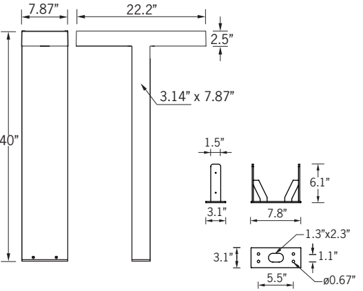
Mounting Detail
